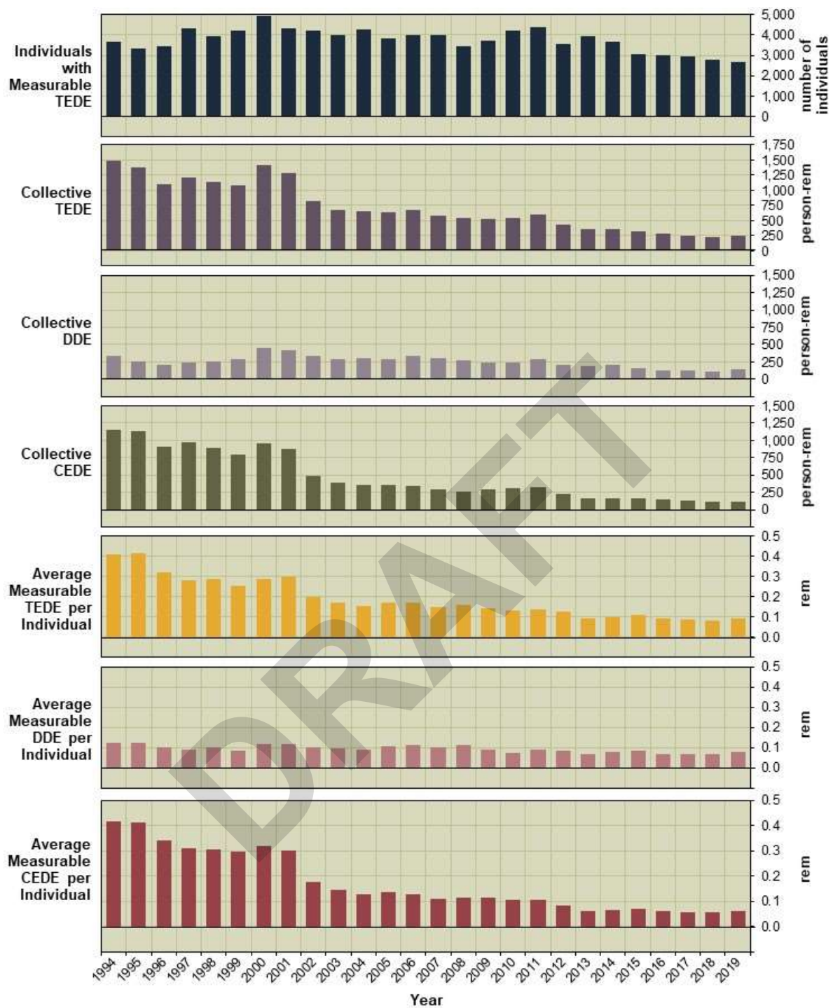
Figure 3.4 Annual Exposure Information for Fuel Cycle Licensees 1994–2019
